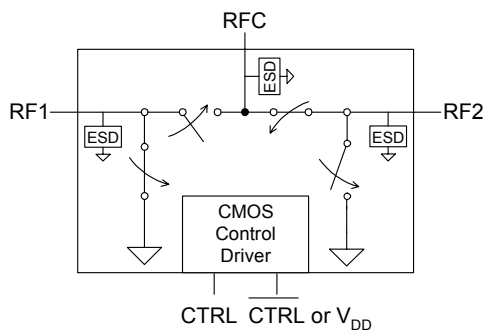
Figure 1. Functional Diagram
