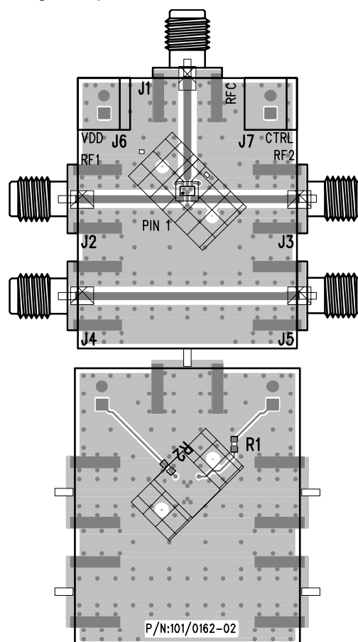
Figure 5. Evaluation Board Layouts Peregrine Specification 101/0162
