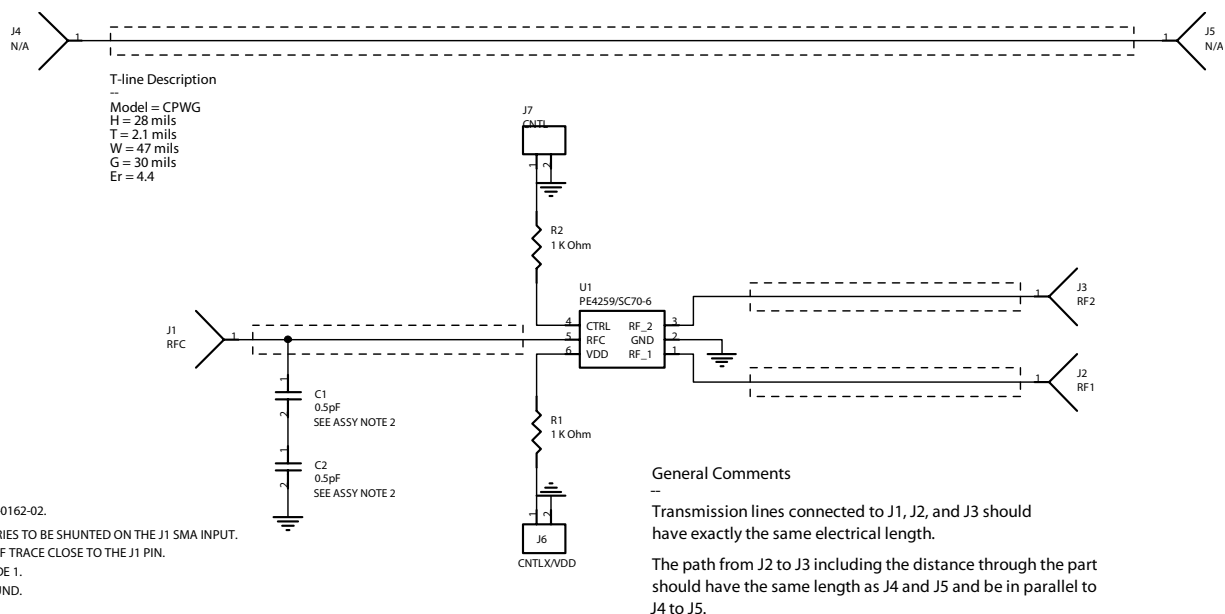
Figure 6. Evaluation Board Schematic Peregrine Specification 102/0218
